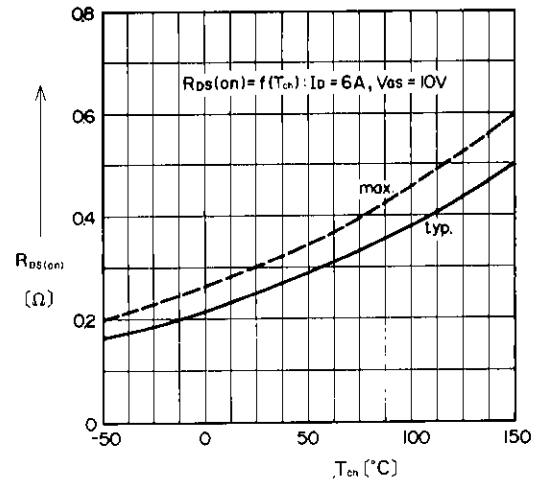
On State Resistance vs. T_{cn}
