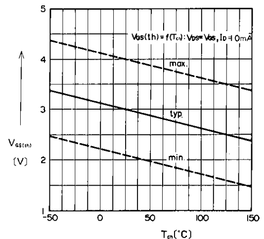
Gate Threshold Voltage vs T_{cn}
