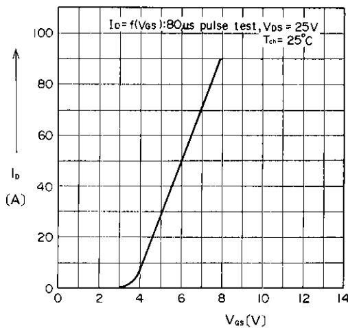
Typical Transfer Characteristic
