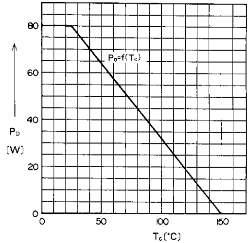
Allowable Power Dissipation vs. T_c
