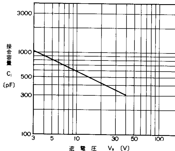
Junction Capacitance Characteristics
