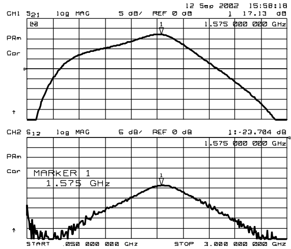
S21,S12
