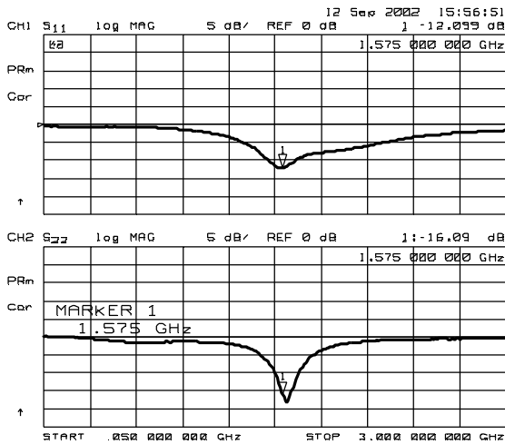
S11,S22
