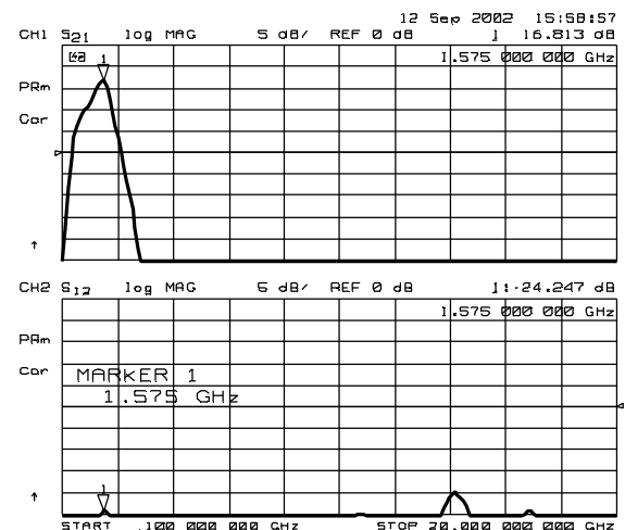
S21, S12(~20GHz)
