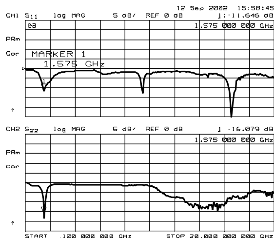
S11, S22(~20GHz)
