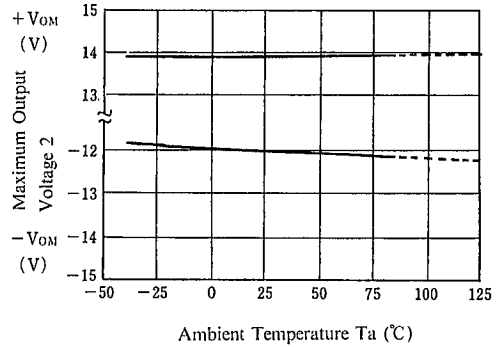
Maximum Output Voltage 2 vs. Temperature
