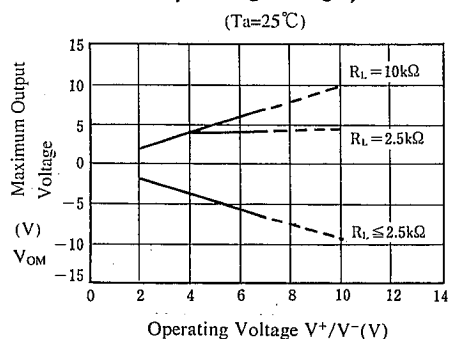
Maximum Output Voltage vs. Operating Voltage
