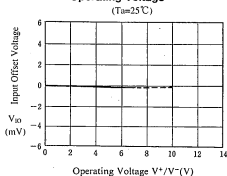
Input Offset Voltage vs. Operating Voltage
