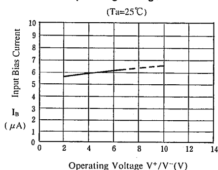
Input Bias Current vs. Operating Voltage
