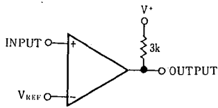
Basic Comparator
