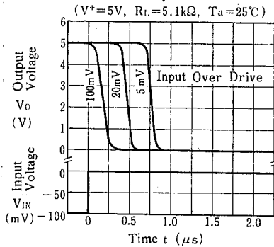
Response Time for Various Input Over Drives ( V^+ = 5\text{ V} , R_L = 5.1\text{ k}\Omega , T_a = 25^\circ\text{C} )
