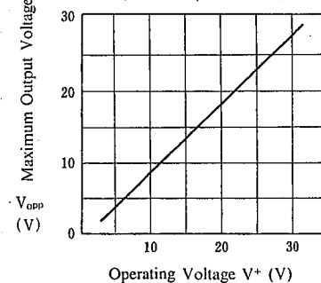
Maximum Output Voltage vs. Operating Voltage
