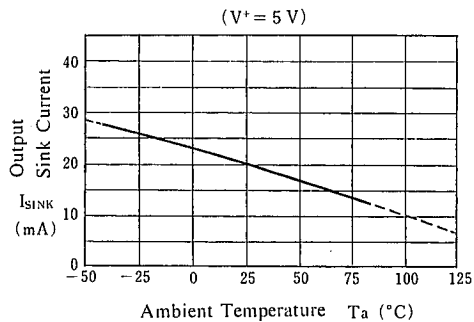
Output Sink Current vs. Temperature
