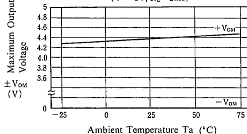
Maximum Output Voltage vs. Temperature
