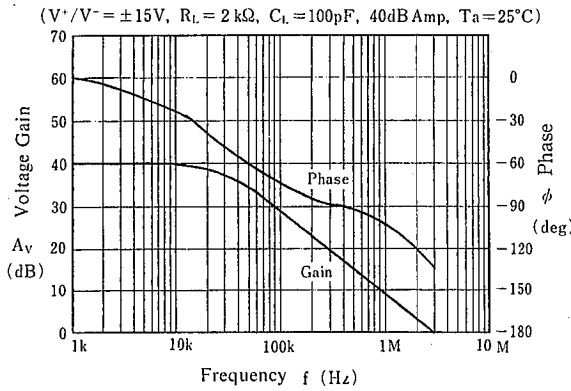
Voltage Gain, Phase vs. Frequency
