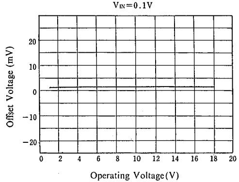
Offset Voltage vs. Operating Voltage
