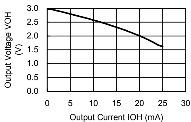
Output Voltage vs. Output Current (Source)
