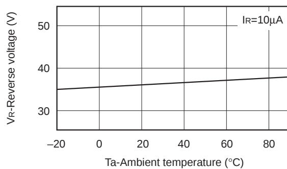
Reverse voltage vs. Ambient temperature
