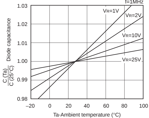
Diode capacitance vs. Ambient temperature f=1\text{MHz}
