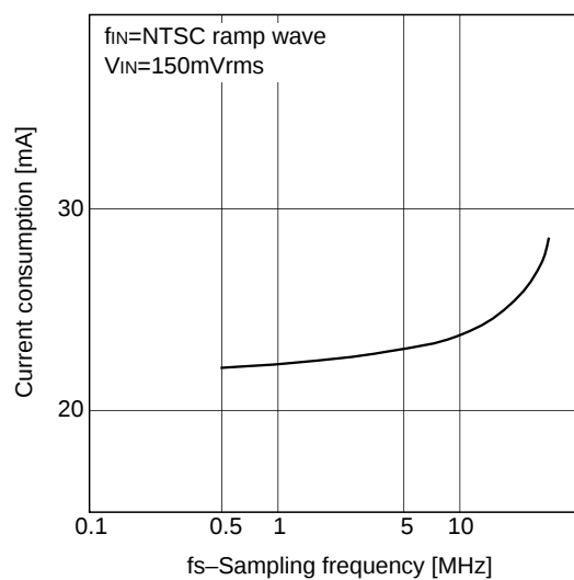
Sampling frequency vs. Current consumption
