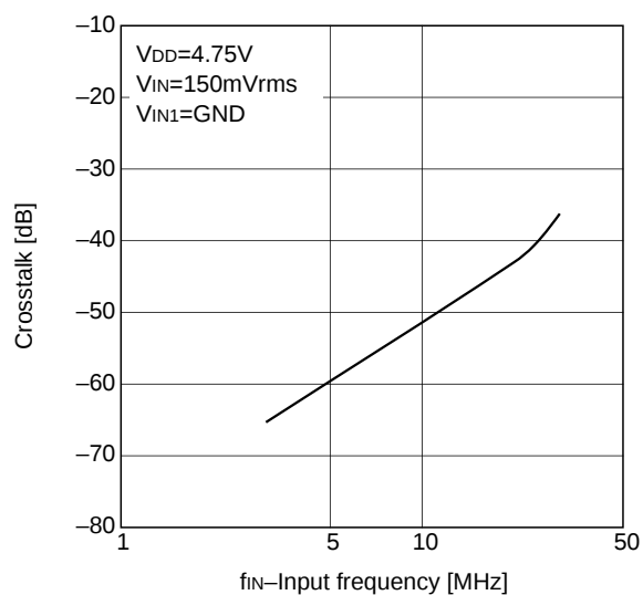
Input frequency of V_{IN2} vs. Crosstalk V_{IN2} \rightarrow V_{IN1}
