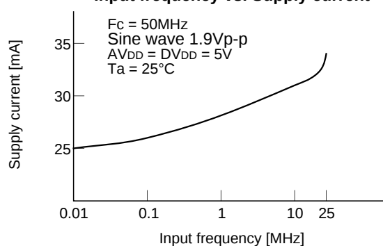
Input frequency vs. Supply current
