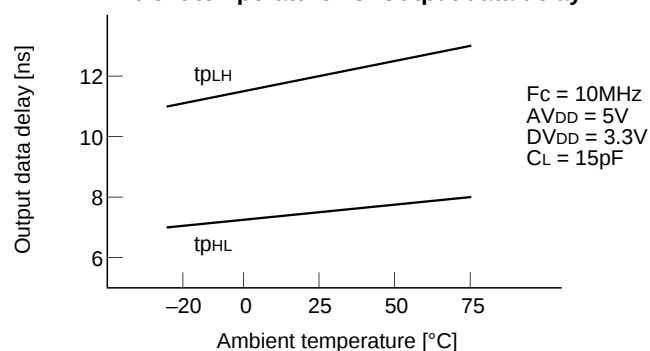
Ambient temperature vs. Output data delay
