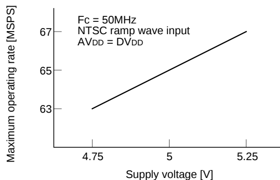
Supply voltage vs. Maximum operating frequency
