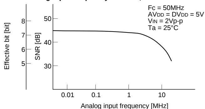
Analog input frequency vs. SNR, effective bit
