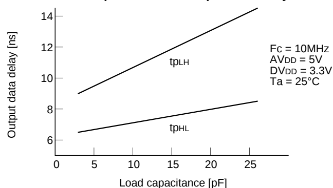
Load capacitance vs. Output data delay
