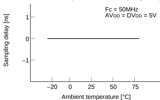
Ambient temperature vs. Sampling delay
