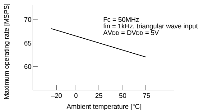
Ambient temperature vs. Maximum operating frequency
