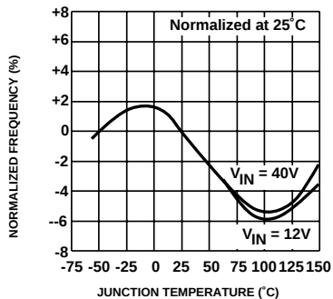
Oscillator Frequency
