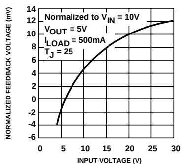
Line Regulation
