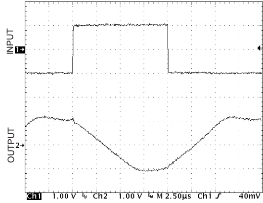
Inverting Large-Signal Pulse Response
