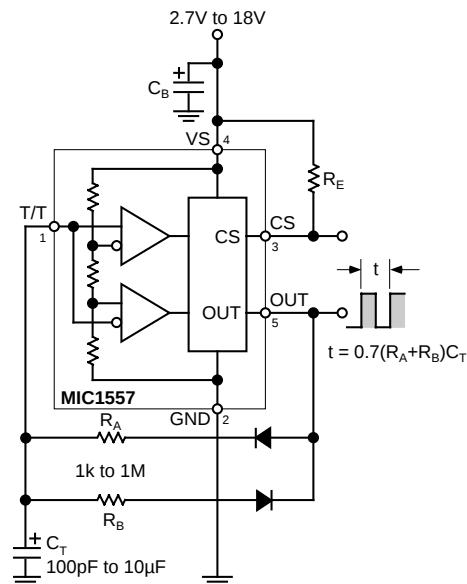
Figure 2. Oscillator Diagram
