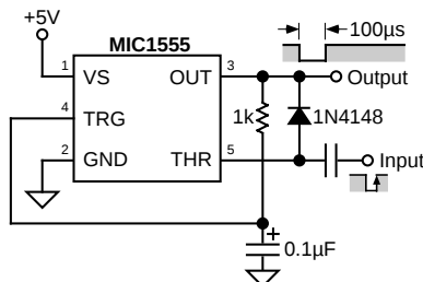
Figure 6. Rising-Edge Trigger Configuration
