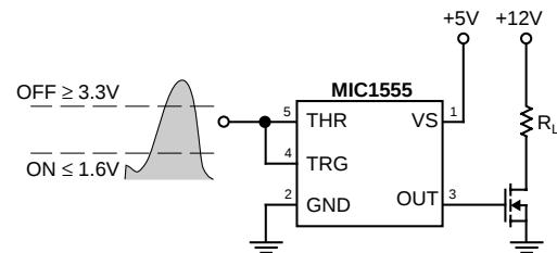
Figure 7. Schmitt trigger
