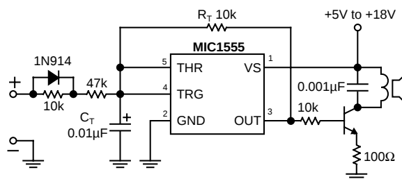
Figure 9. Audible Voltmeter
