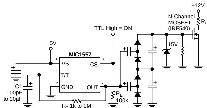
Figure 8. Charge-Pump
