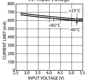
Short-Circuit Current-Limit vs. Input Voltage
