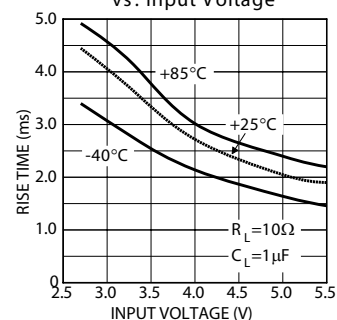
Turn-On Rise Time vs. Input Voltage
