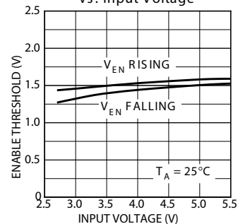
Enable Threshold vs. Input Voltage
