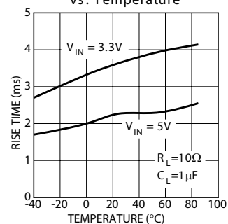
Turn-On Rise Time vs. Temperature
