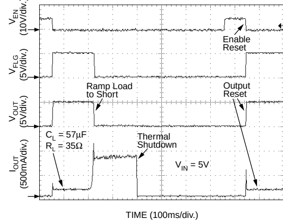
Thermal Shutdown (Output Reset by Toggling Enable—MIC2076-2)
