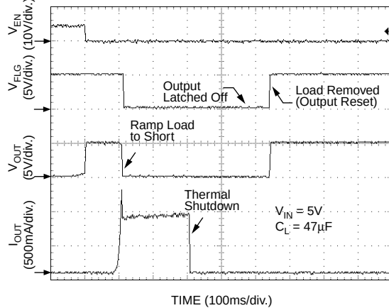
Thermal Shutdown (Output Reset by Removing Load—MIC2076-2)
