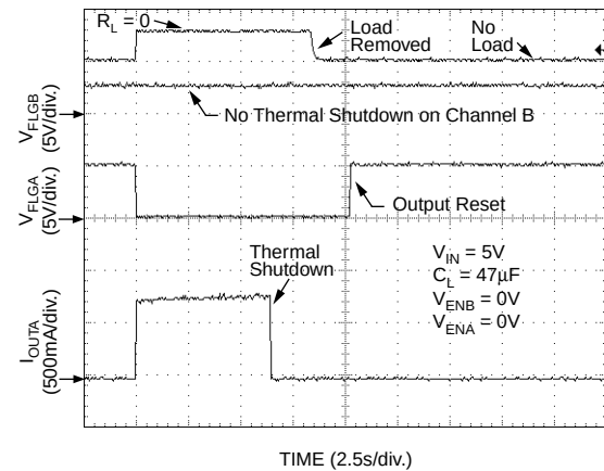
Independent Thermal Shutdown (MIC2076-2)
