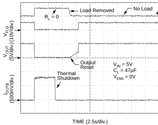
Thermal Shutdown (MIC2076-2—Output Latched Off)
