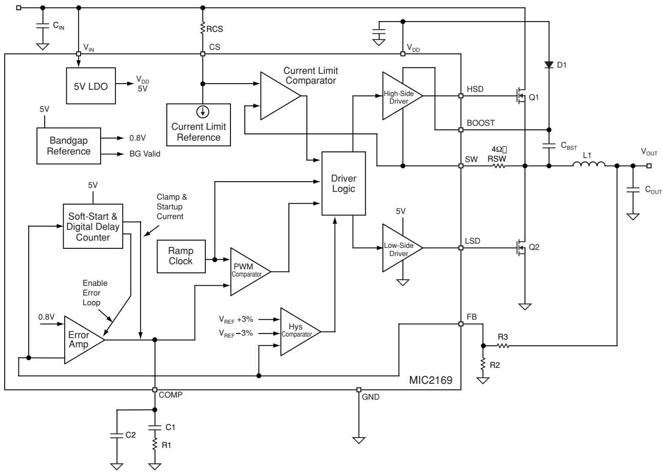
MIC2169 Block Diagram
