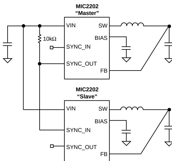
Figure 1. Master-Slave Operation
