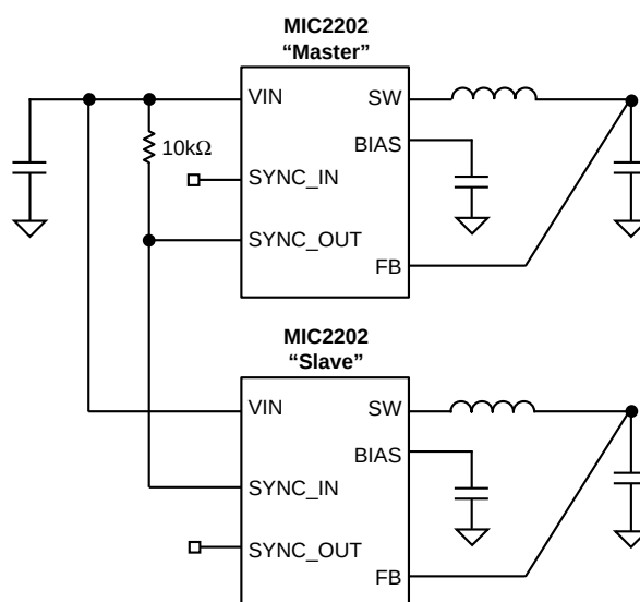
Figure 4. Master-Slave Operation
