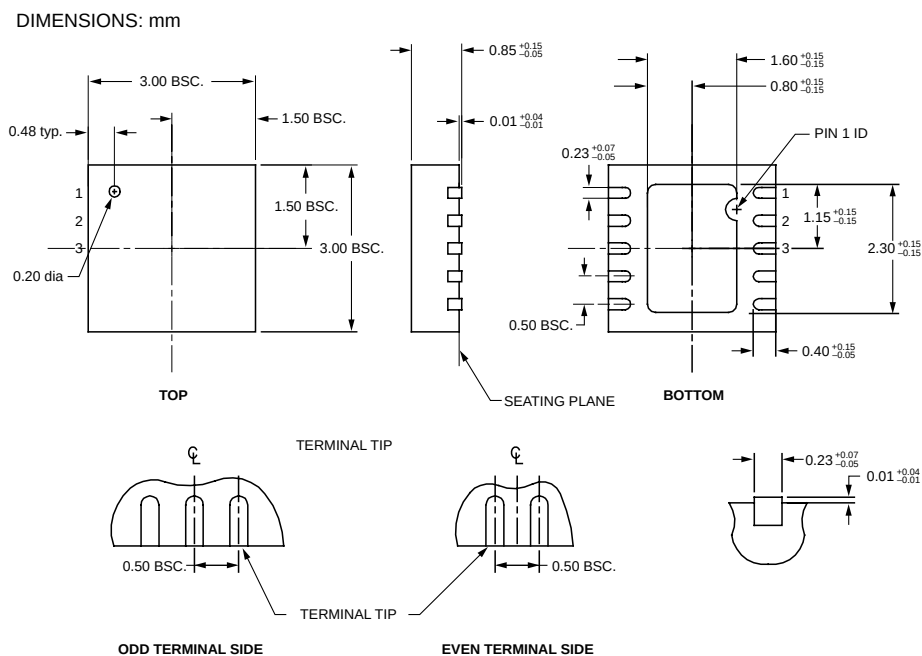
10-Pin MLF™ (ML)
