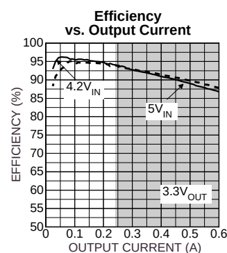
Figure 2. Efficiency Curve
