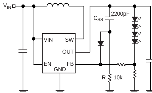
Figure 4. One of Soft-Start Circuit
