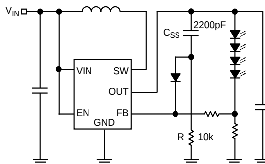
Figure 4. Soft-Start Circuit
