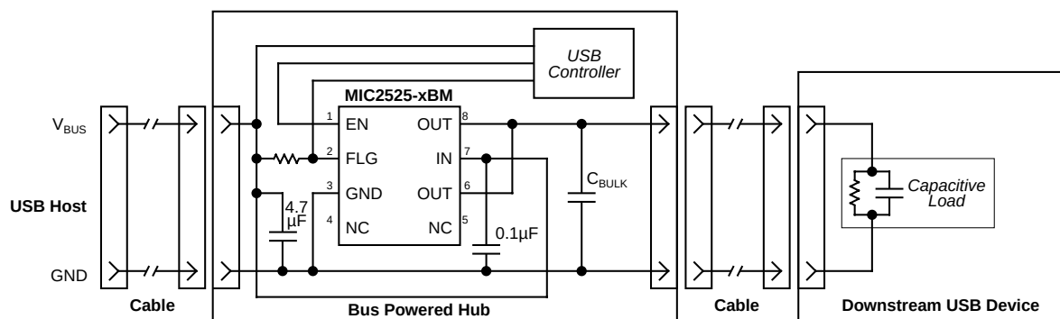
Figure 2. Soft-Start Application
