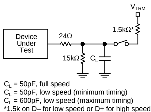
Figure 7. D+ and D— Load
