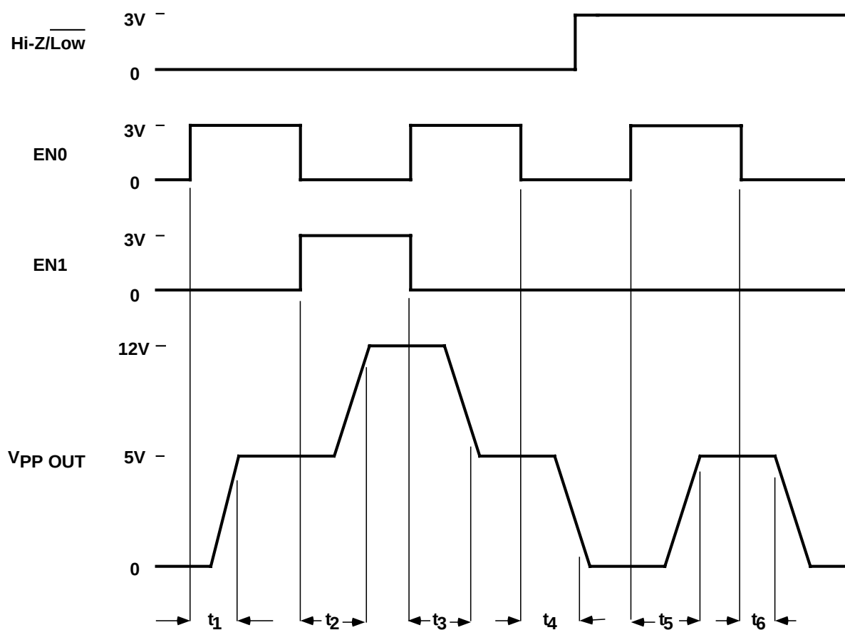
Figure 1. Timing Diagram.
