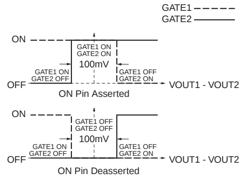
Figure 2. Gate Voltage Window — Tracking Mode
