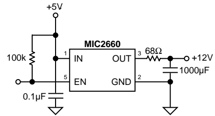
Figure 2. Charge-Pump/Dump
