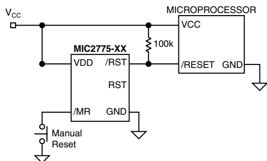
Figure 1. MIC2775 Valid /Reset Below 1.2V
