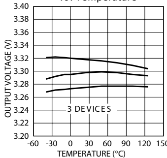
MIC29750-3.3 Output Voltage vs. Temperature
