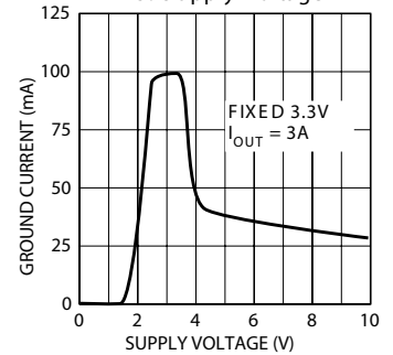
MIC2930x Ground Current vs. Supply Voltage
