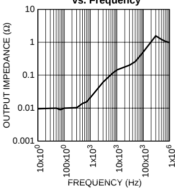
MIC2975x Output Impedance vs. Frequency
