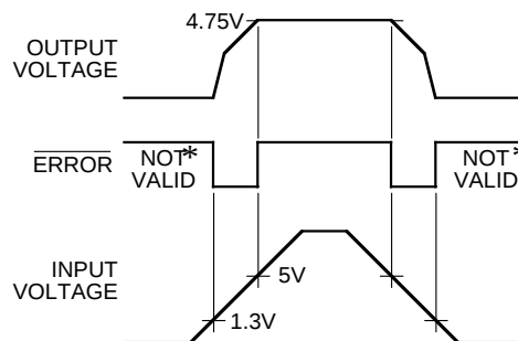
Figure 1. ERROR Output Timing
