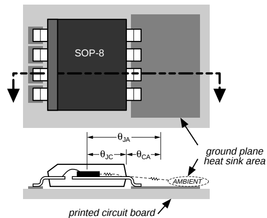
Figure 3. Thermal Resistance
