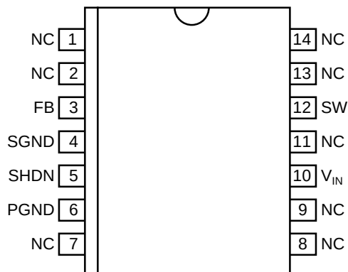
14-Lead Wide SOIC (WM)
