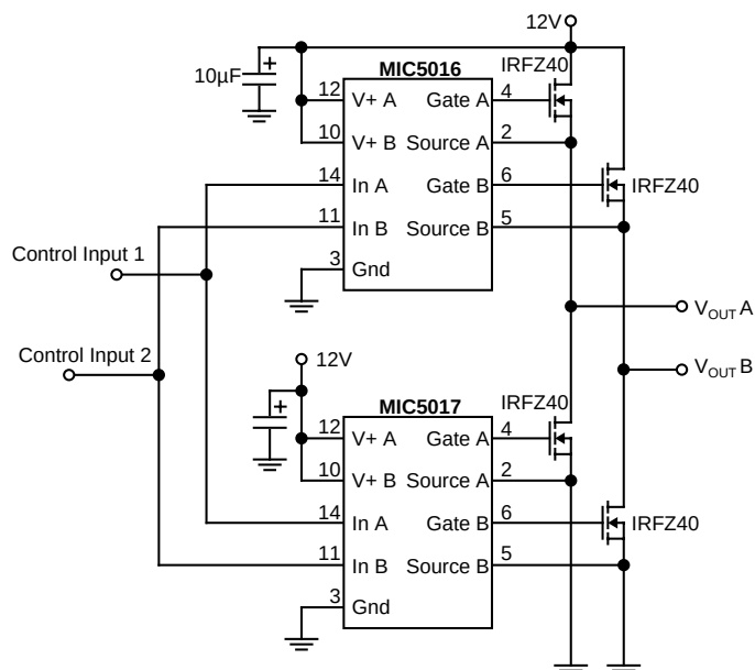
Figure 13: Push-Pull Driver
