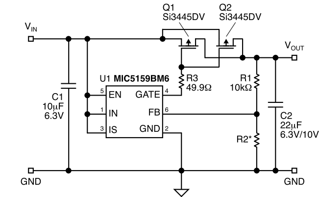
Application Circuit
