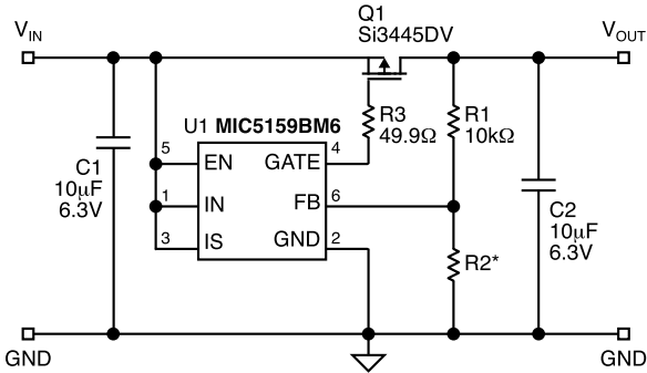
Application Circuit
