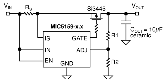
Figure 4. Adjustable Regulator Design
