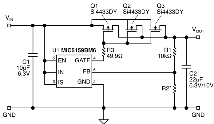
Application Circuit
