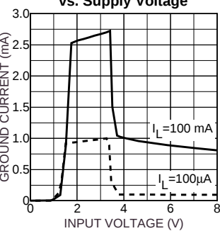
Ground Current vs. Supply Voltage
