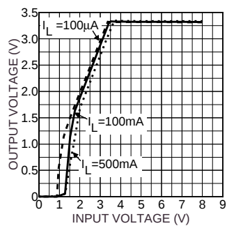
Dropout Characteristics
