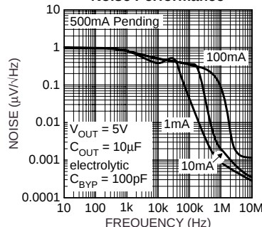
Noise Performance
