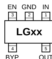
MIC5219-x.xBM5 SOT-23-5 Fixed Voltages
