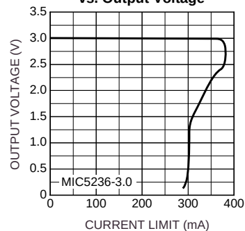
Current Limit vs. Output Voltage
