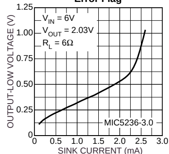
Current Limit Induced Error Flag
