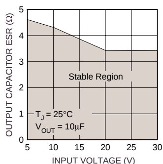
Figure 2. Output Capacitor ESR
