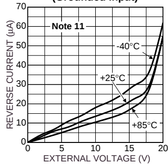
Reverse Current (Grounded Input)
