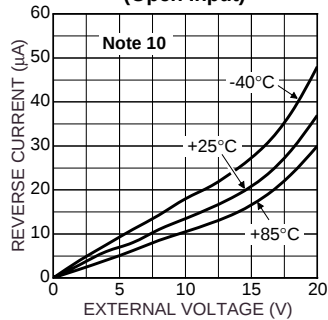
Reverse Current (Open Input)
