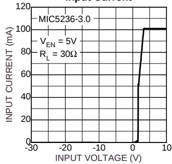
Input Current
