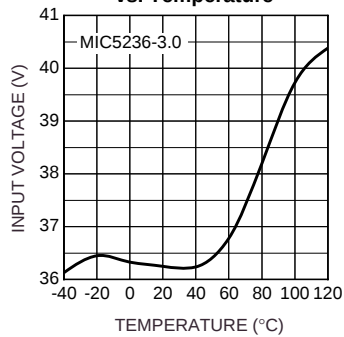
Overvoltage Threshold vs. Temperature
