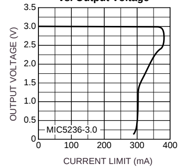
Current Limit vs. Output Voltage
