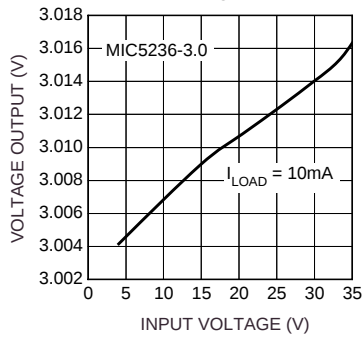
Line Regulation
