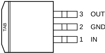
MIC5237-x.xBU (TO-263-3)
