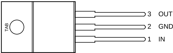
MIC5237-x.xBT (TO-220-3)
