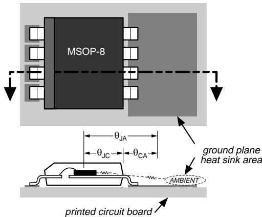
Figure 5. Thermal Resistance
