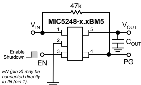
Low-Noise Regulator Application
