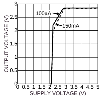
Dropout Characteristics
