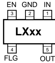
MIC5256-x.xBM5 (SOT-23-5)
