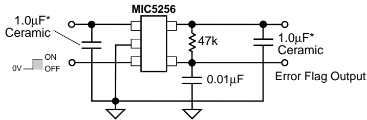
Figure 1. Test Circuit
